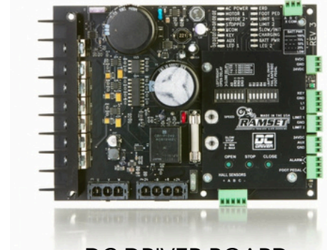
DC DRIVER BOARD
