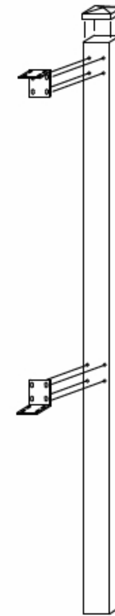
120x120x4mm (5"x5"x5/32") 9' Long Heavy Wall Post
