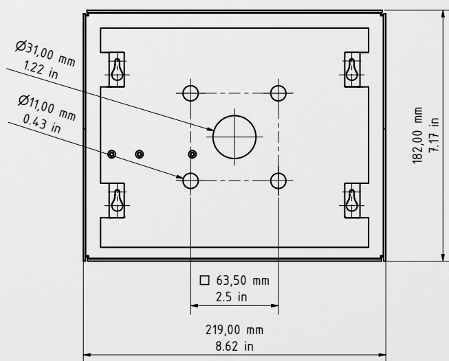
Housing (backbox)
