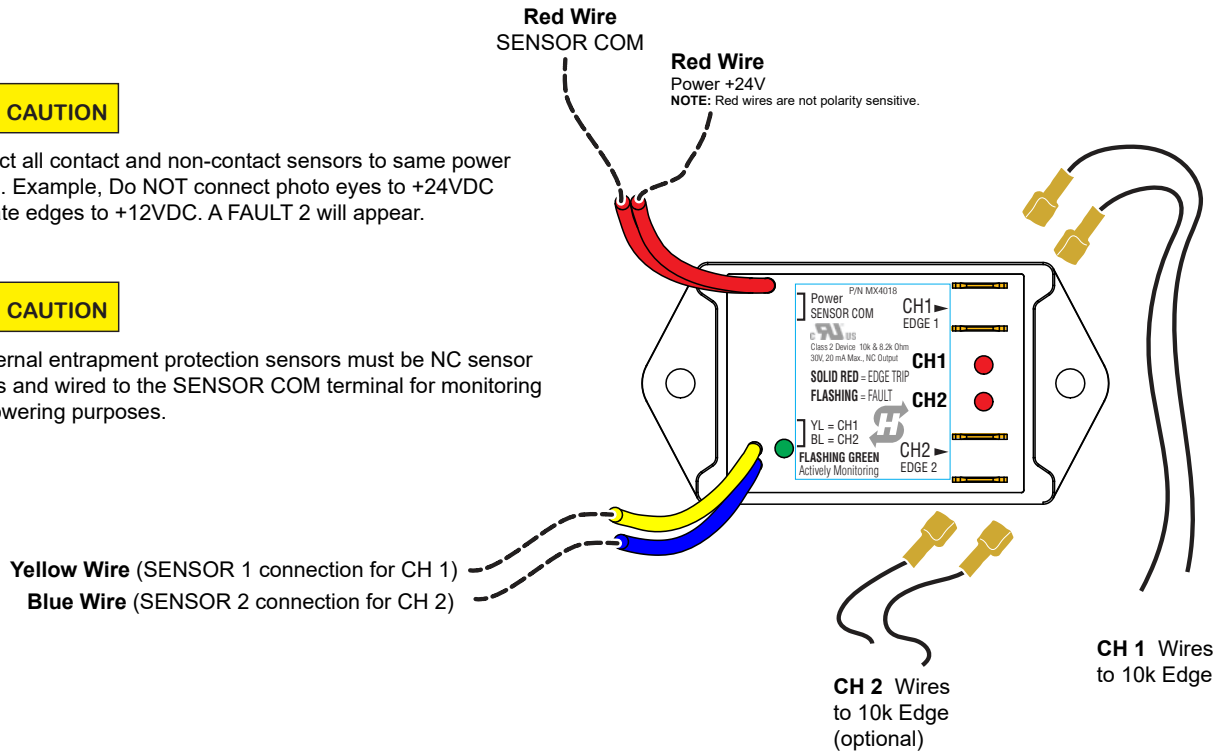
HY2NC Wiring Diagram
