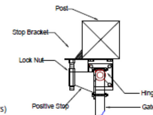
120x120x4mm (4-3/4"x4-3/4"x5/32") 7' Long Heavy Wall Post
