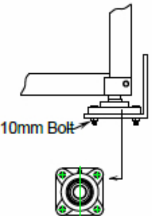
Super Duty Sealed Bearing Hinge W/Adjustable Bracket
