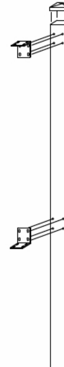
120x120x4mm (5"x5"x5/32") 9' Long Heavy Wall Post
