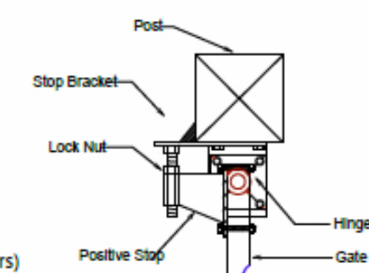
120x120x4mm (5"x5"x5/32") 9' Long Heavy Wall Post
