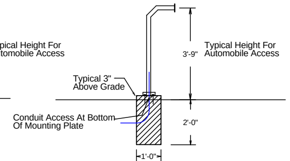
Pad Mount Style Gooseneck
