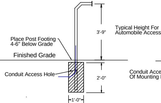
Post Style Gooseneck
