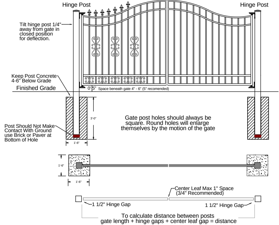
Dual Gate (Bi-parting)
